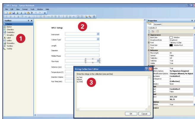
Figure 3: Graphical Form Designer.
